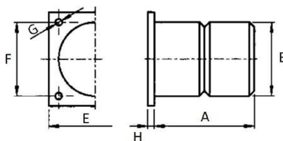
PLATE FIXED ZELLPUFFER
